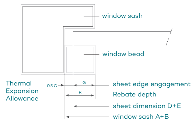
Figure 13: Thermal Expansion allowance of LEXAN sheet in the glazing profiles
