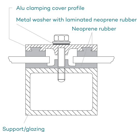
Figure 28: LEXAN sheet installation by using aluminum clamping profile
