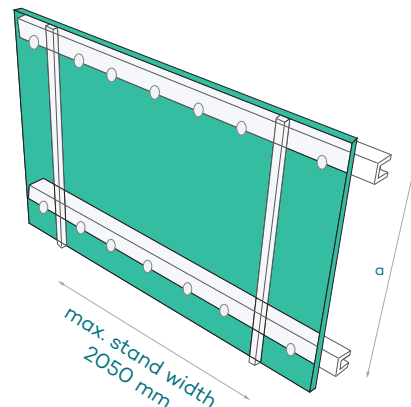
Figure 24: Using conventional nuts, bolts and washers to fasten LEXAN sheet.
