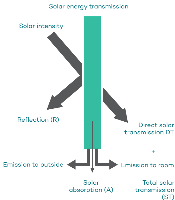
Figure 6: Solar Energy Transmission
