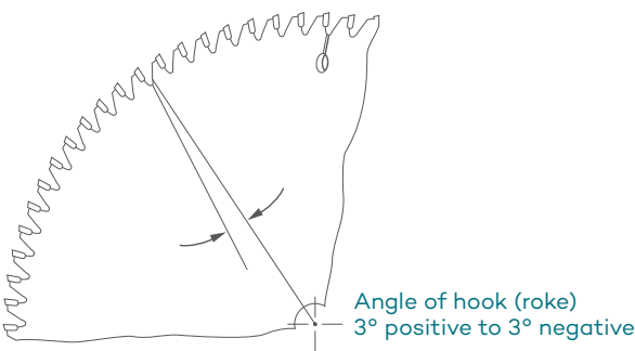
Figure 8: Tungsten carbide tipped saw blades used for circular saws
