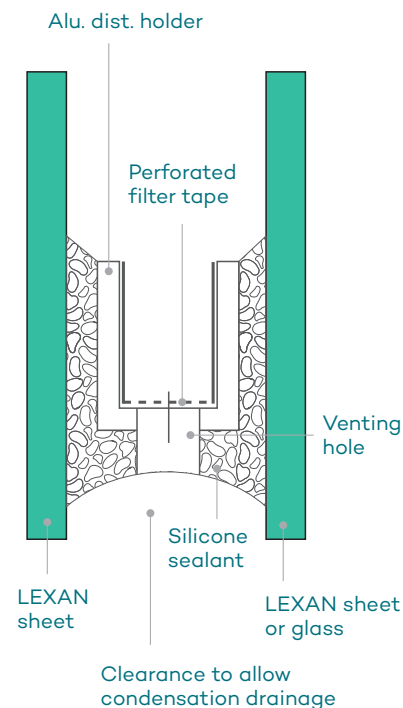
Figure 20: Double Glazing Units
