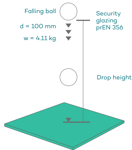
Figure 3: Steel Ball Impact Test
