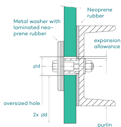
Figure 25: Fixation of LEXAN sheet to support/ glazing profile with metal washers and bolts.
