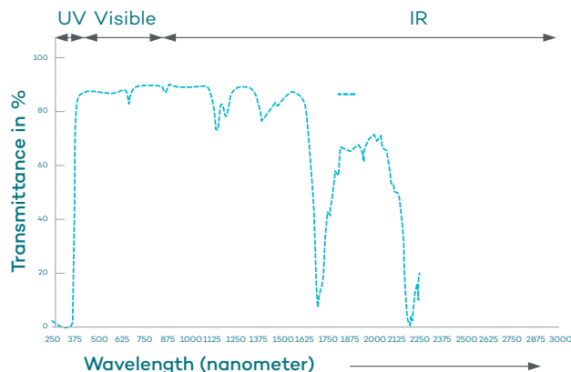
Figure 5: Light Transmission Spectrum of LEXAN sheet
