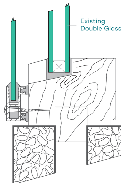
Figure 19: External Overglazing
