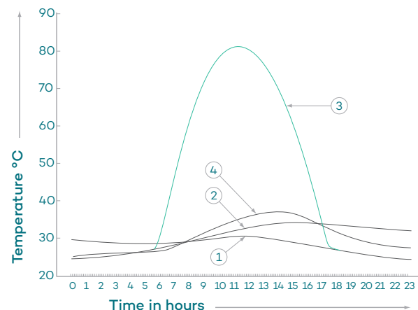
Figure 7: Free-blown Domes during a day
