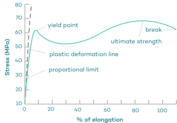
Figure 1: Stress-strain diagram for solid LEXAN sheet
