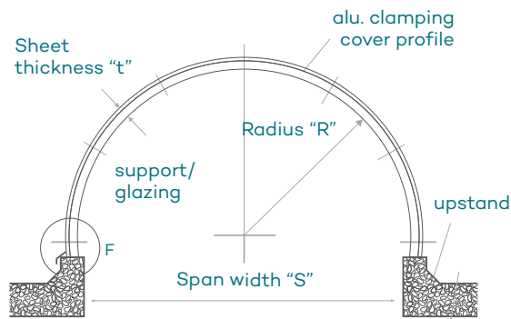
Figure 26: Curving of LEXAN sheet
