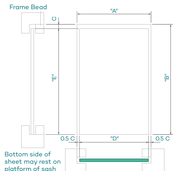
Figure 12: The minimum required sheet edge engagement of LEXAN sheet in the glazing profiles
