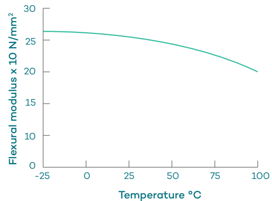
Figure 2: Flexural modulus vs temperature
