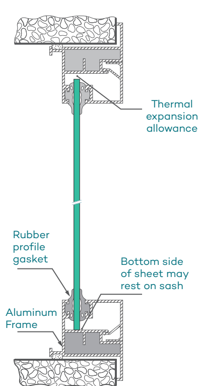
Figure 14: Dry glazing installation
