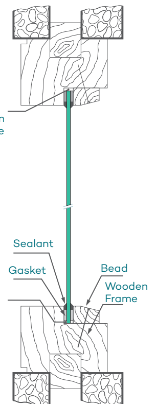
Figure 15: Wet glazing installation
