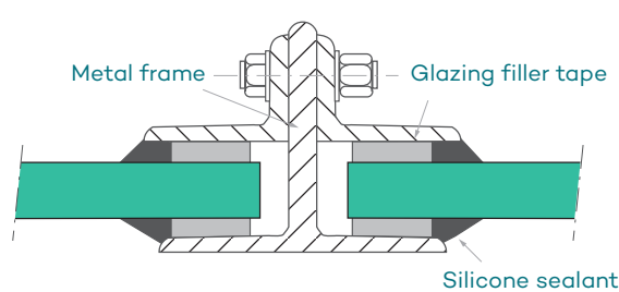
Figure 27: Wet Glazing
