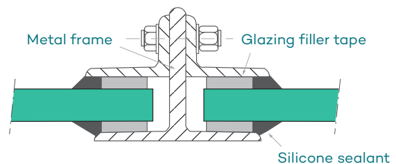
Figure 16: Wet Glazing
