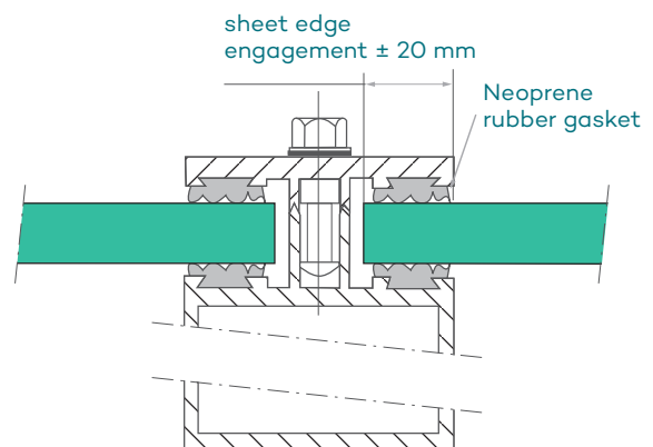
Figure 17: Dry Glazing
