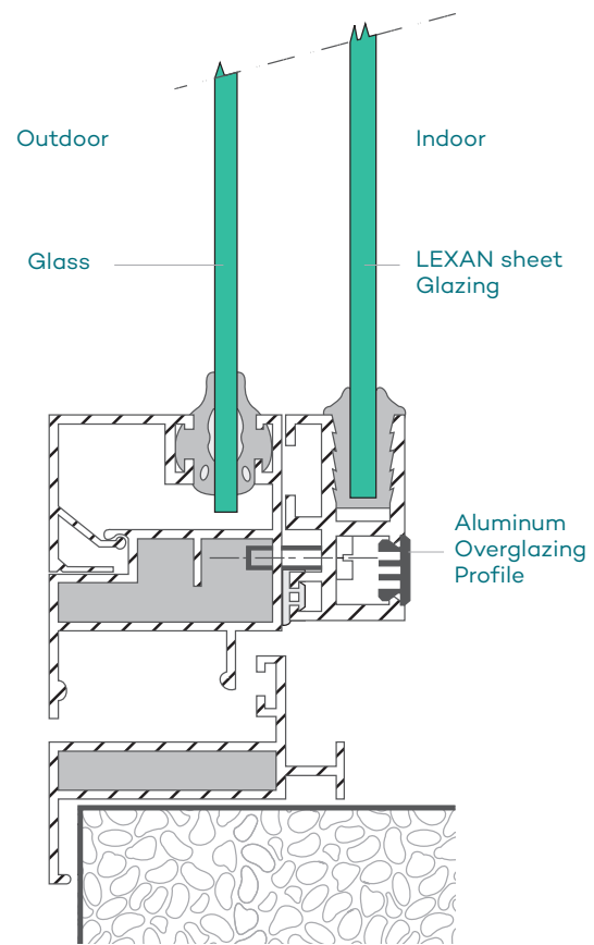
Figure 18: Internal Overglazing
